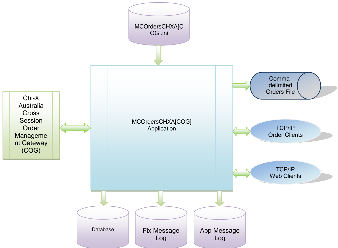
Figure 1. The MCOOrdersCHXA[COG] Production System
